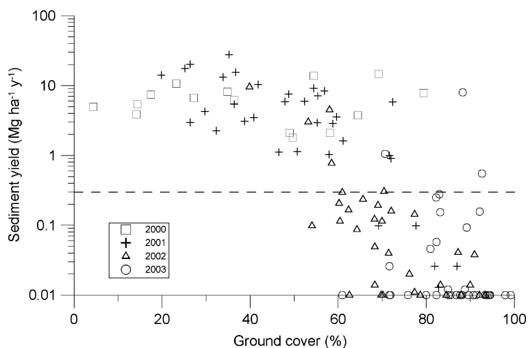
Figure 6. Plot of annual sediment yields versus ground cover for 2000–03. Each point represents one year of data from one plot ( n = 117 ). The 29 plots with little or no sediment were assigned values of 0.01 \text{ Mg ha}^{-1} \text{ year}^{-1} . The dashed line represents the assumed background sediment yield of 0.3 \text{ Mg ha}^{-1} \text{ year}^{-1} .
